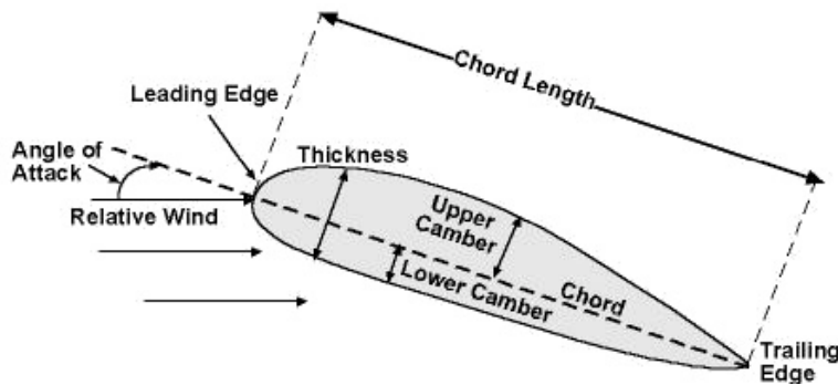
The angle of attack is the angle between the chord of the airfoil and the relative wind.
