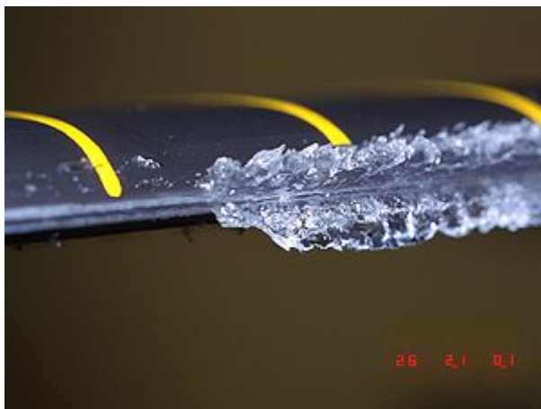
Ice protrusions on the rotor blade
